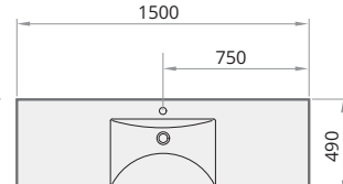
LONG STEP 1500/C
